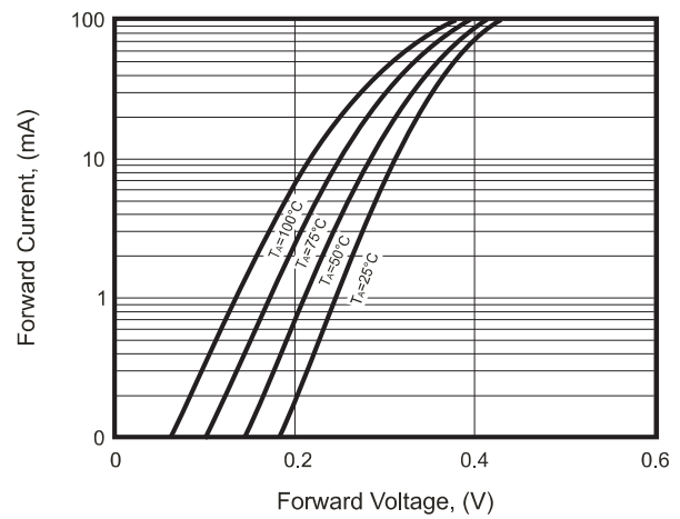
Fig.2 - Forward Characteristics
